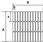
Domino Mosaic A 11 21/32" B 11 49/64" a 4" b 1"
