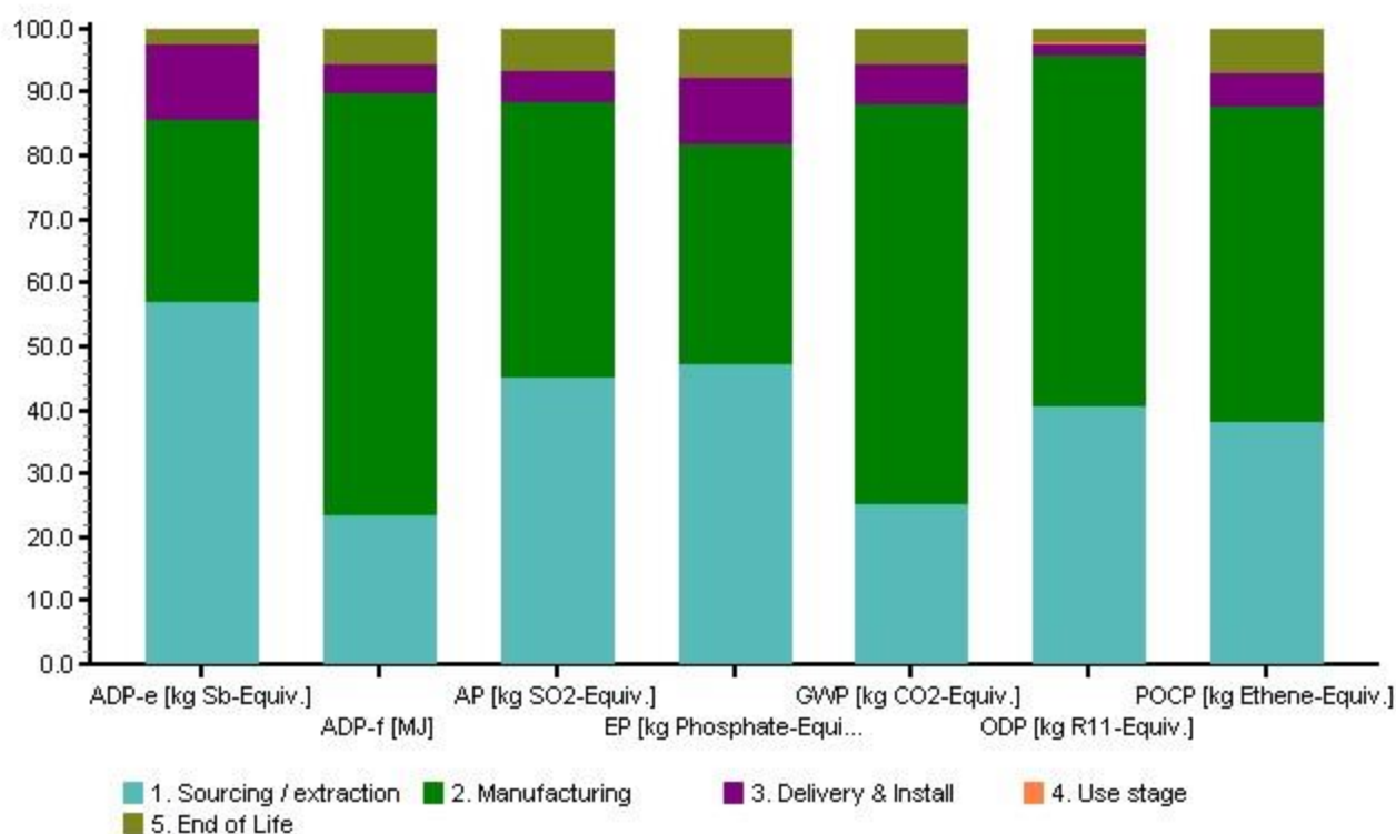
Figure 3: CML Impact assessment results of 1 square meter for 1 year use
