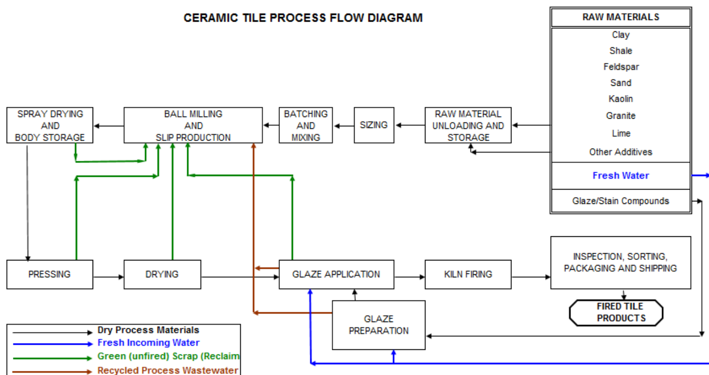
Figure 6: Process flow diagram for tile manufacturing – no fired scrap
