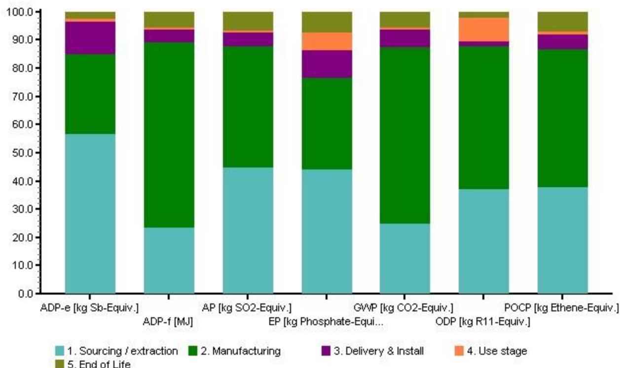
Figure 4: CML Impact assessment results of 1 square meter for 60 year use
