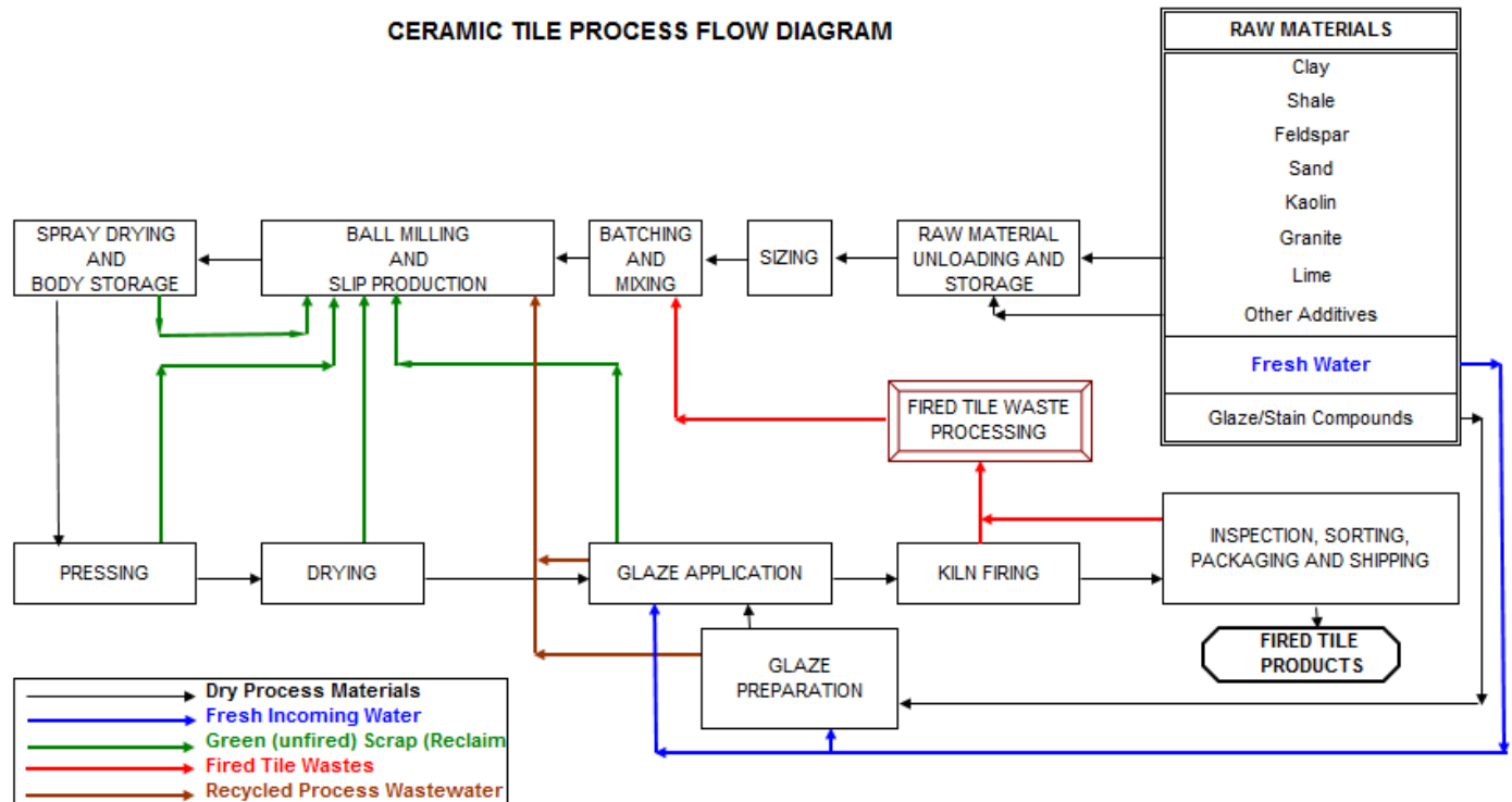
Figure 7: Process flow diagram for tile manufacturing – with recycled fired scrap
